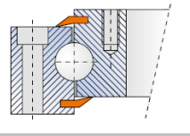
4-point contact ball bearing
